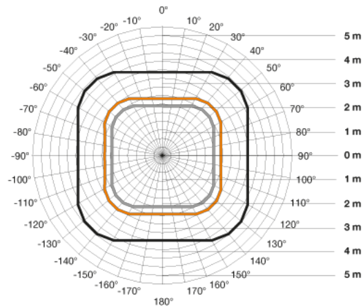
Presence Control PRO IR Quattro, installation height 2.8 m (black = tangential, orange = radial, grey = presence)
